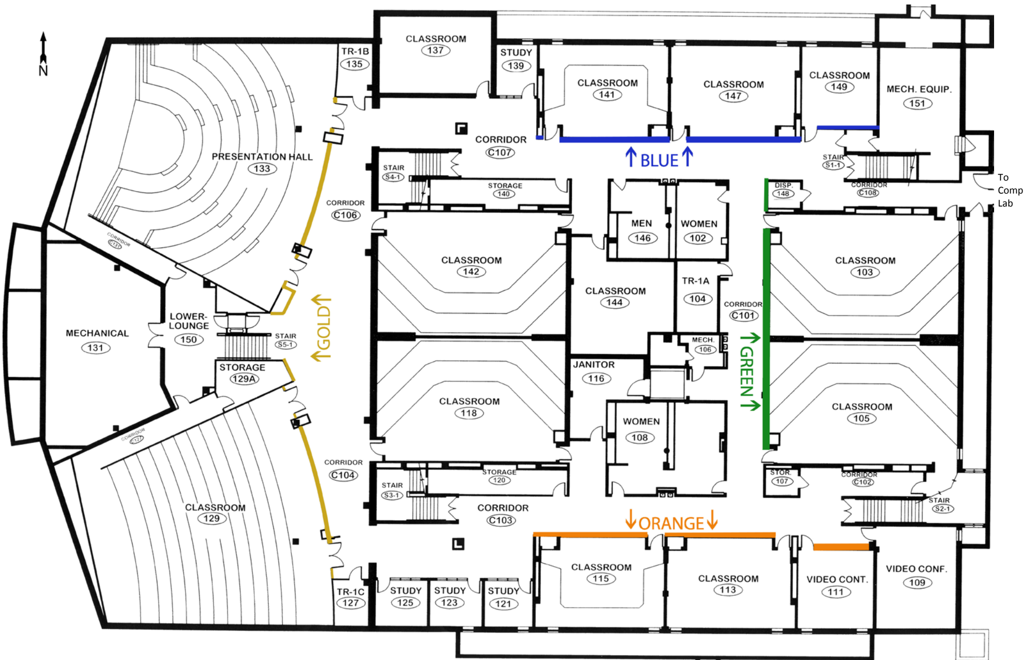
Classroom Building Basement Level
